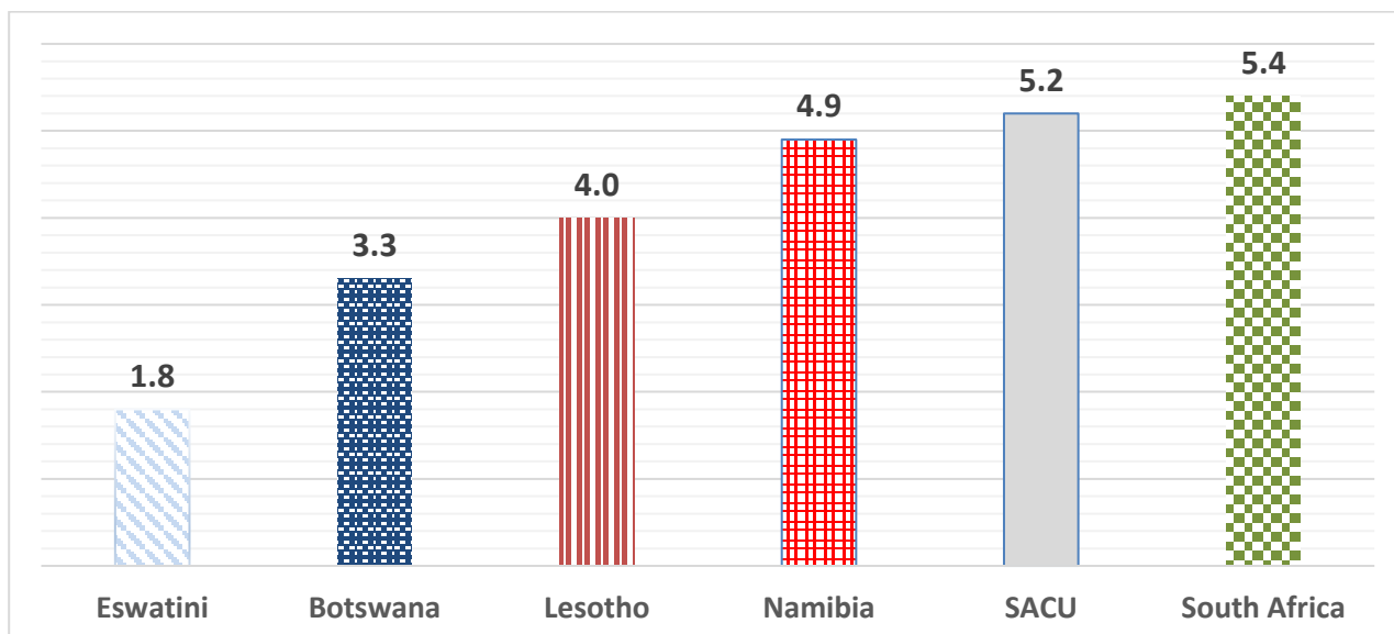
Chart I: Annual inflation rates (%) in May 2019, in ascending order
