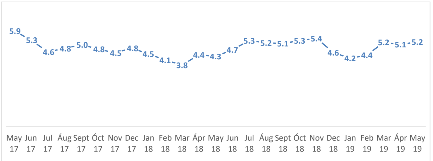
Chart 2: Annual inflation rates (%) in SACU
